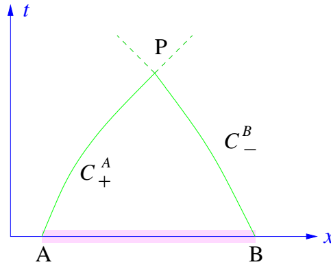
Non-linear characteristic curves.
