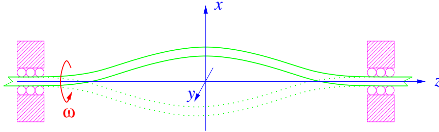
The n = 1 even-parity mode of a whirling shaft.
