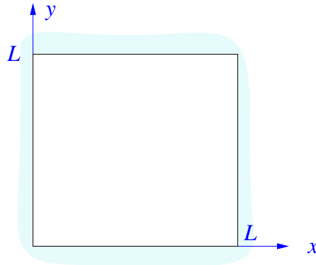
Square region.
