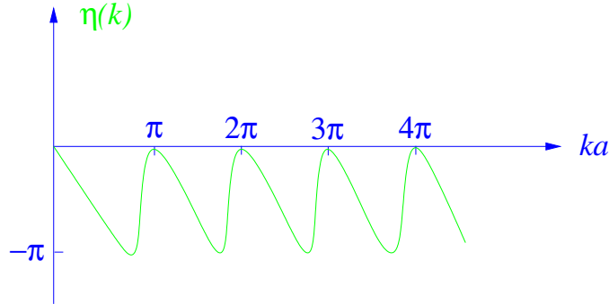
Phase shift as a function of k .
