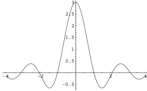
A plot of \pi\delta_{\Lambda}^{\text{F}}(x) for \Lambda = 3 .
