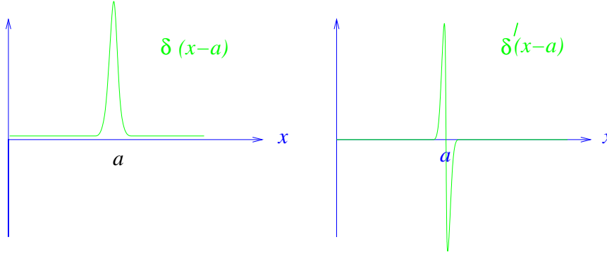
Smooth approximations to \delta(x-a) and \delta'(x-a) .
