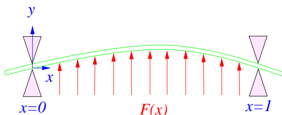
Simply supported rod.
