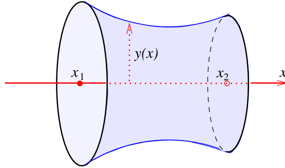
Soap film between two rings.
