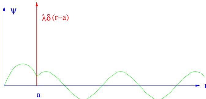
Delta function shell potential.
