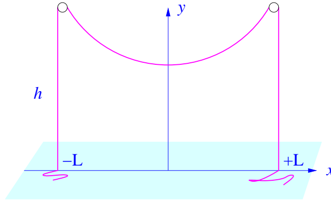
Hanging chain.
