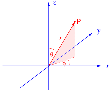
Spherical co-ordinates.
