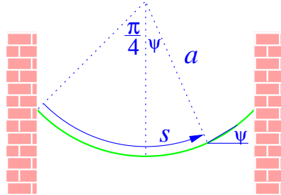
Weighted line.
