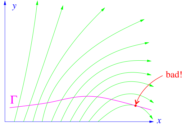
Initial data curve \Gamma , and flow-line characteristics.
