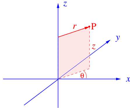
Cylindrical co-ordinates.
