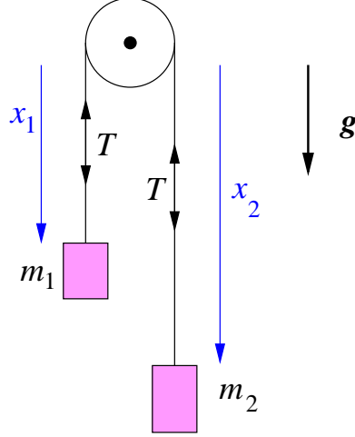
Atwood's machine.
