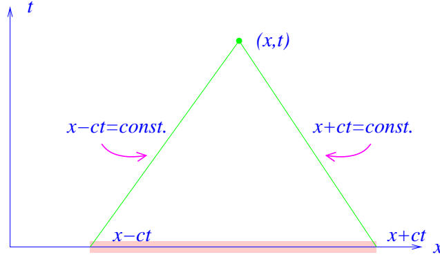
Range of Cauchy data influencing \varphi(x, t) .
