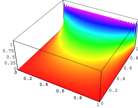
Plot of first thirty terms in (6.141).
