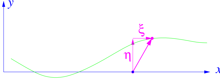
Vibrating piano string.
