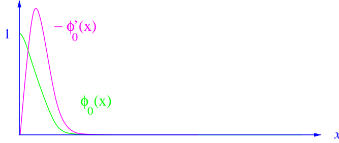
The function \phi_0(x) and its derivative.
