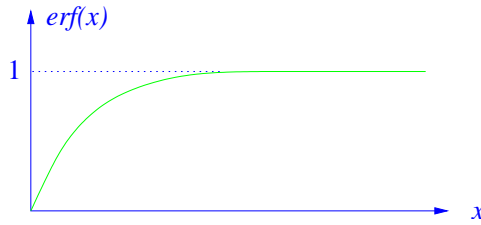
Error function.
