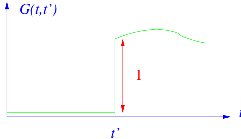
The Green function G(t, t') for the first-order initial value problem .
