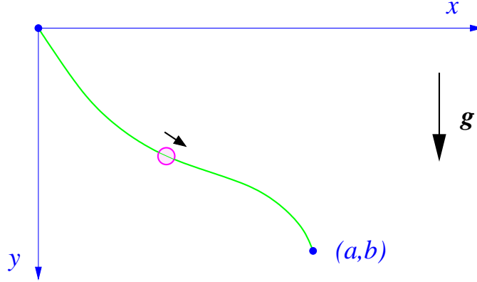
Bead on a wire.
