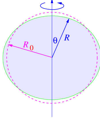
Deformed planet.
